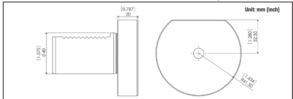
Protection Plug
