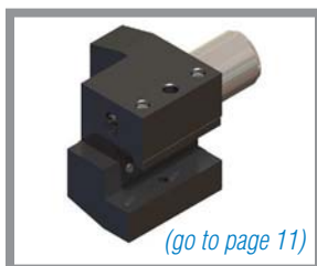
Part #: VDI40-BG15Z-C-E2 Double External Coolant Flow Boring Bar Holder
