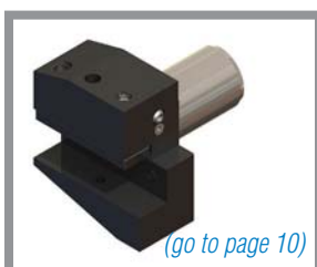
Part #: VDI40-ID10Z-C2 Left Hand Axial Turning Tool
