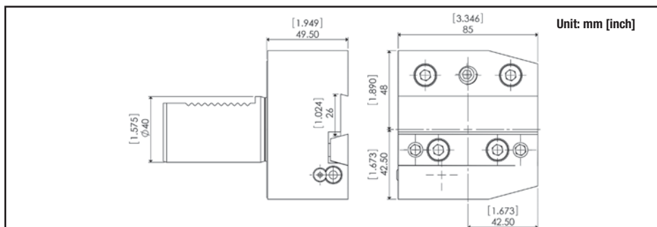
Cut Off Tool
