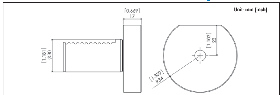
Protection Plug
