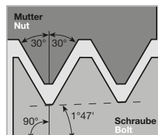
NPTF - Vollprofil NPTF - Full Profile
