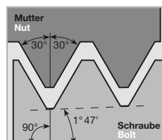
NPT - Vollprofil NPT - Full Profile
