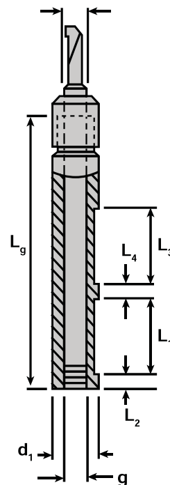
4, 6, & 8mm MicroBore Shank Sizes
