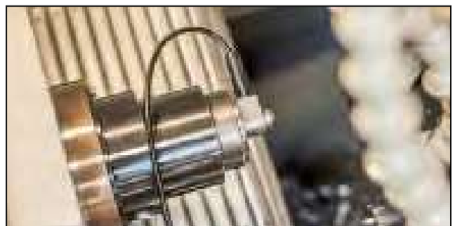
Camera in sub spindle
