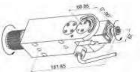
DE20-0004 Angled Drilling / Milling Collet Size: ER11 Output: 1:1 Coolant-Thru (Ext) Adjustable 0-90°
