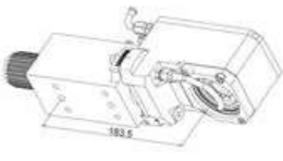
DE20-W15-II Thread Whirling Ring: Utilis Output: 1:1 9 or 12 Insert Cutter, Flight Circle Ø12mm Coolant-Thru (Ext)
