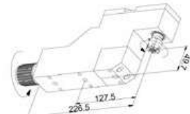
DE20-0011 Drilling / Milling Collet Size: ER16 Output: 1:1
