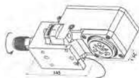
DE13-W15 Thread Whirling Ring: Utilis Output: 1:1 9 or 12 insert cutter, Flight Circle Ø12mm, Uses 2 Tooling Positions Adjustable ±15° Coolant-Thru
