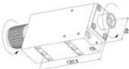
DE20-0002-CR Drilling / Milling Collet Size: ER11 to ER20 Output: 1:1 Length 187mm Coolant-Thru (Ext) Quick Change
