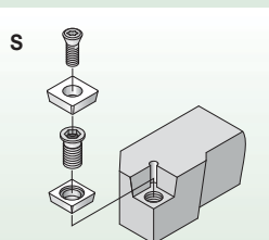
Center clamping by screw for inserts with hole.
