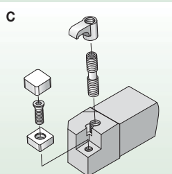
Top clamping by clamping finger for inserts without hole.
