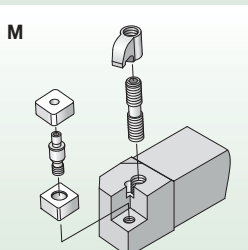
Top and hole clamping for inserts with hole.
