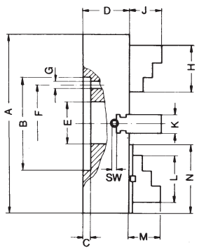
Cylindrical centre mount
