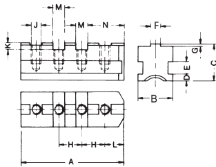
Base jaw GB
