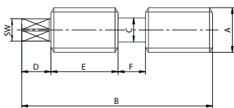
Adjusting spindle
